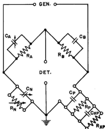
Figure 5. Substitution Parallel-Resistance Method.
