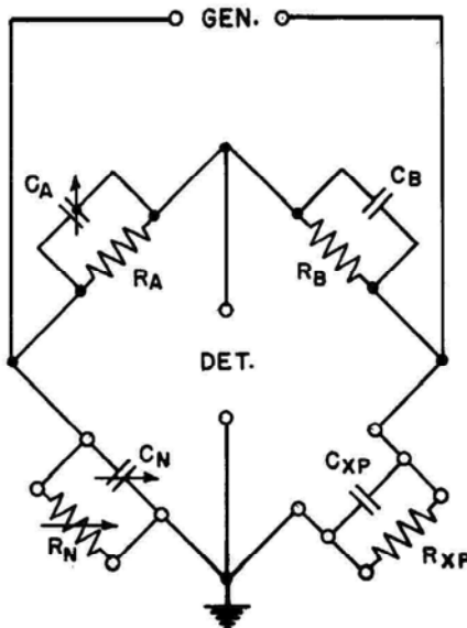
Figure 4. Parallel-Resistance Method.
