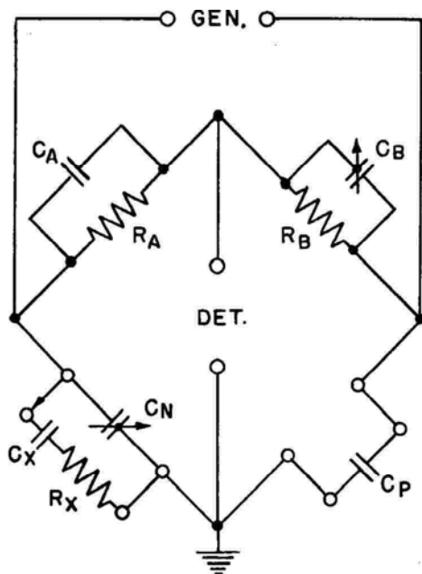
Figure 2. Substitution Method.
