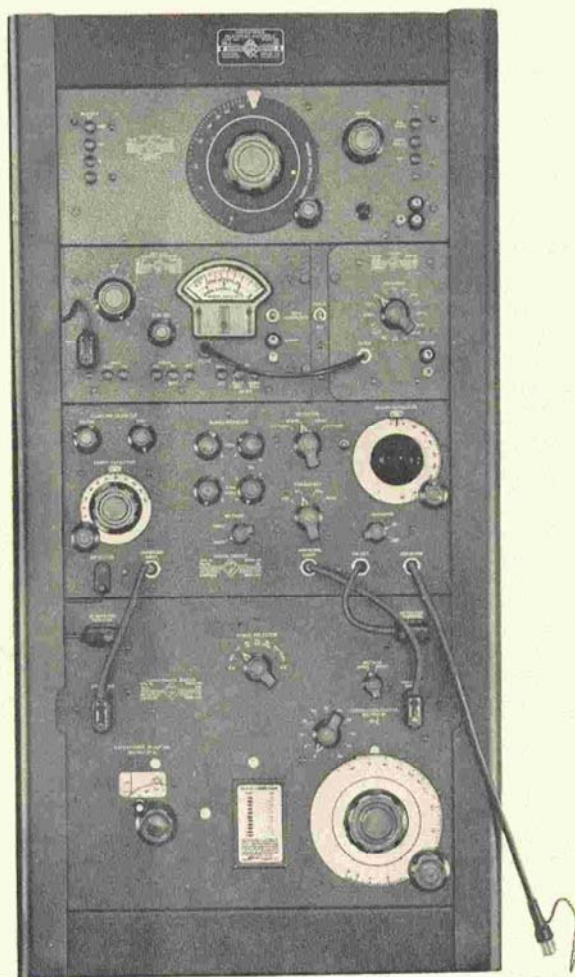
Figure 6. View of Type 1610-A Capacitance Measuring Assembly: Type 1302-A Oscillator, Type 1231-BR Amplifier and Null Detector with Type 1231-P5 Filter, Type 716-P4R Guard Circuit, and Type 716-CR Capacitance Bridge.
